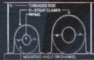
Installation with Rubber support Insert
